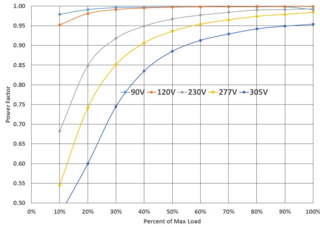
Figure 11. Power Factor
